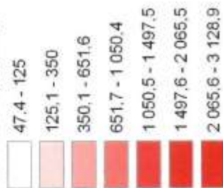
MAX SO2 (ug/m3)
