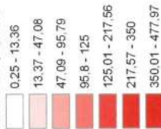
AVG SO2 (ug/m3)
