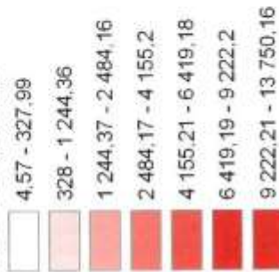
AVG CO (µg/m 3 )
